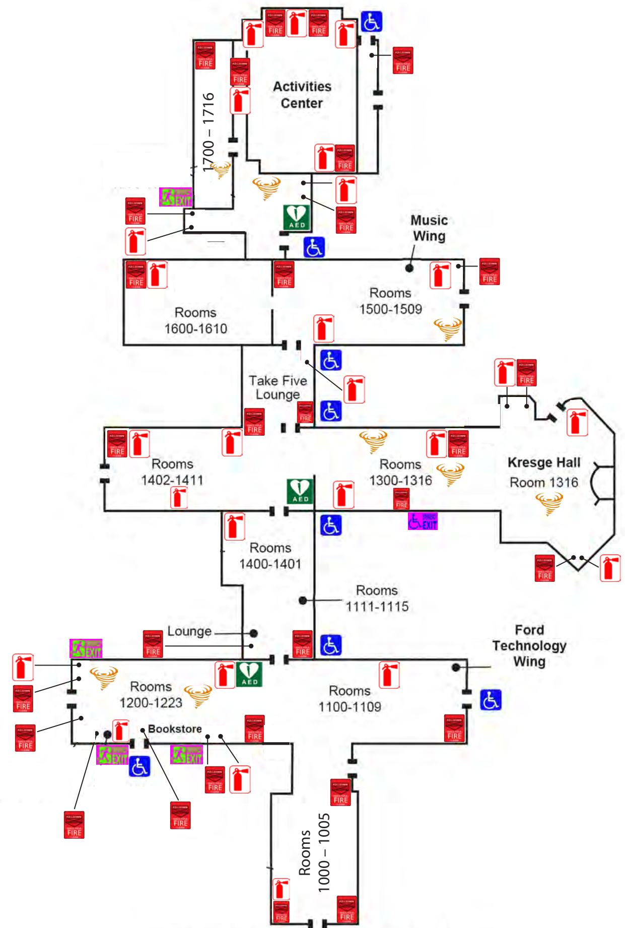
ADMINISTRATION BUILDING FIRST FLOOR
